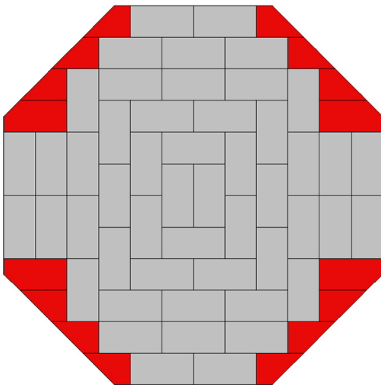
Lay-up instruction wrestling mat 12 x 12 m
